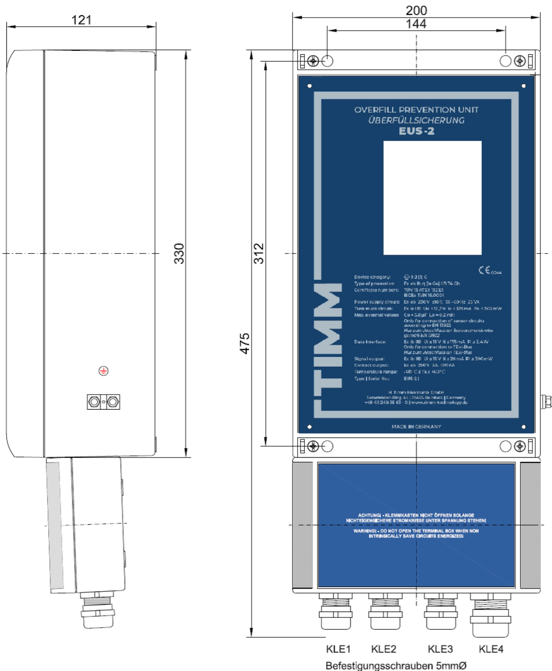
1. Dimensional Drawing
